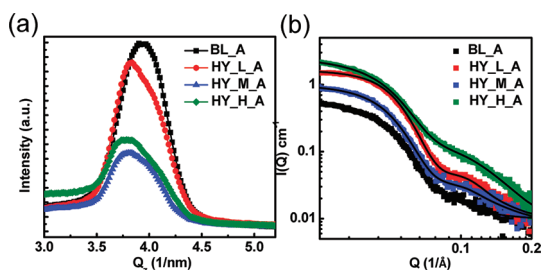
Figure 5. (a) GIWAXS and (b) GISAXS profiles of the annealed P3HT/PCBM blended film (BL_A), and P3HT/PCBM/Cu 2 S INPs hybrid films (HY_L_A, HY_M_A, and HY_H_A). The solid lines represent the fitted GISAXS intensities.
